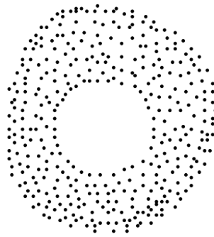
Figure 2.10: Invalid Center
