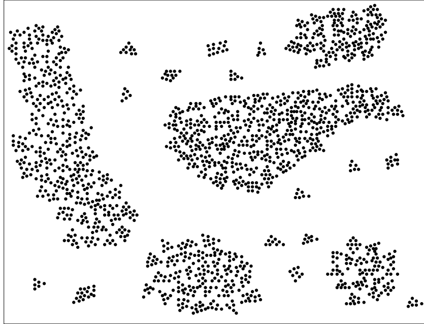
Figure 3.12: Generated Points
