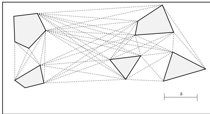
Figure 3.7: Visibility Graph
